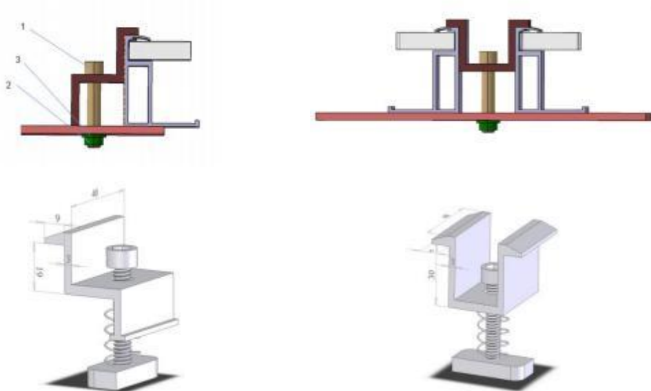
Fig. 2 clamps fixed module
