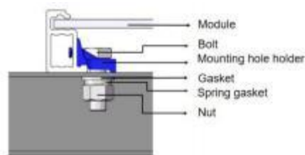
Sectional view
